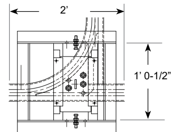
Universal Switch LH-65528 (shown) RH-65529
