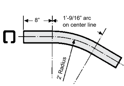
2'-0" RAD. 30° Upper Vertical Curve 20111
