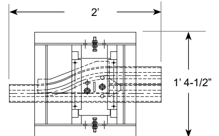
Universal Switch LH-65528 (shown) RH-65529
